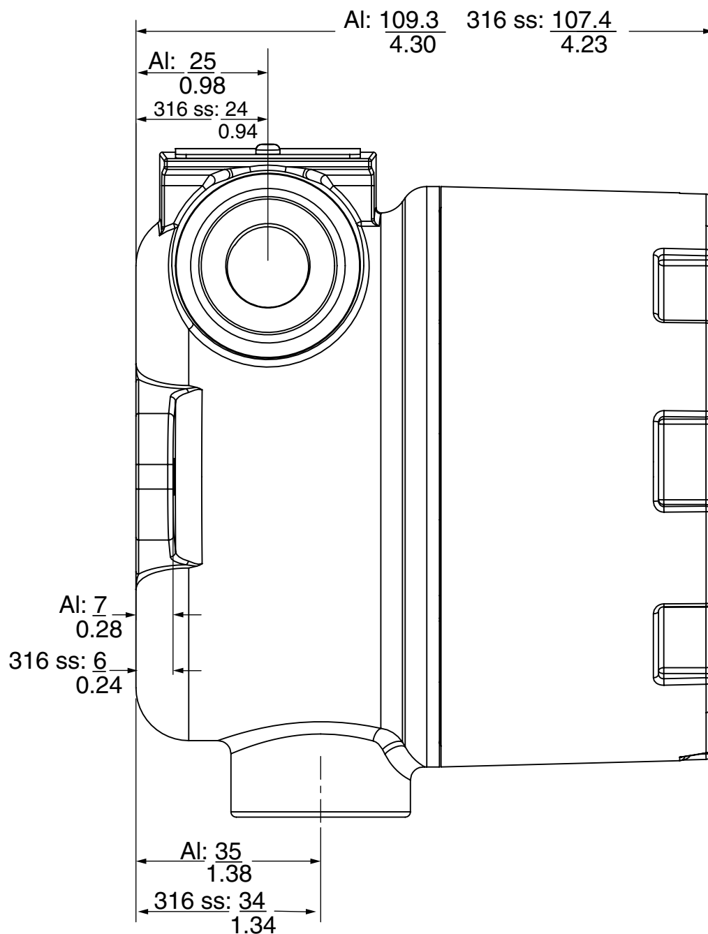
Figure 8 - Transmitter with Display Housing — Side View
