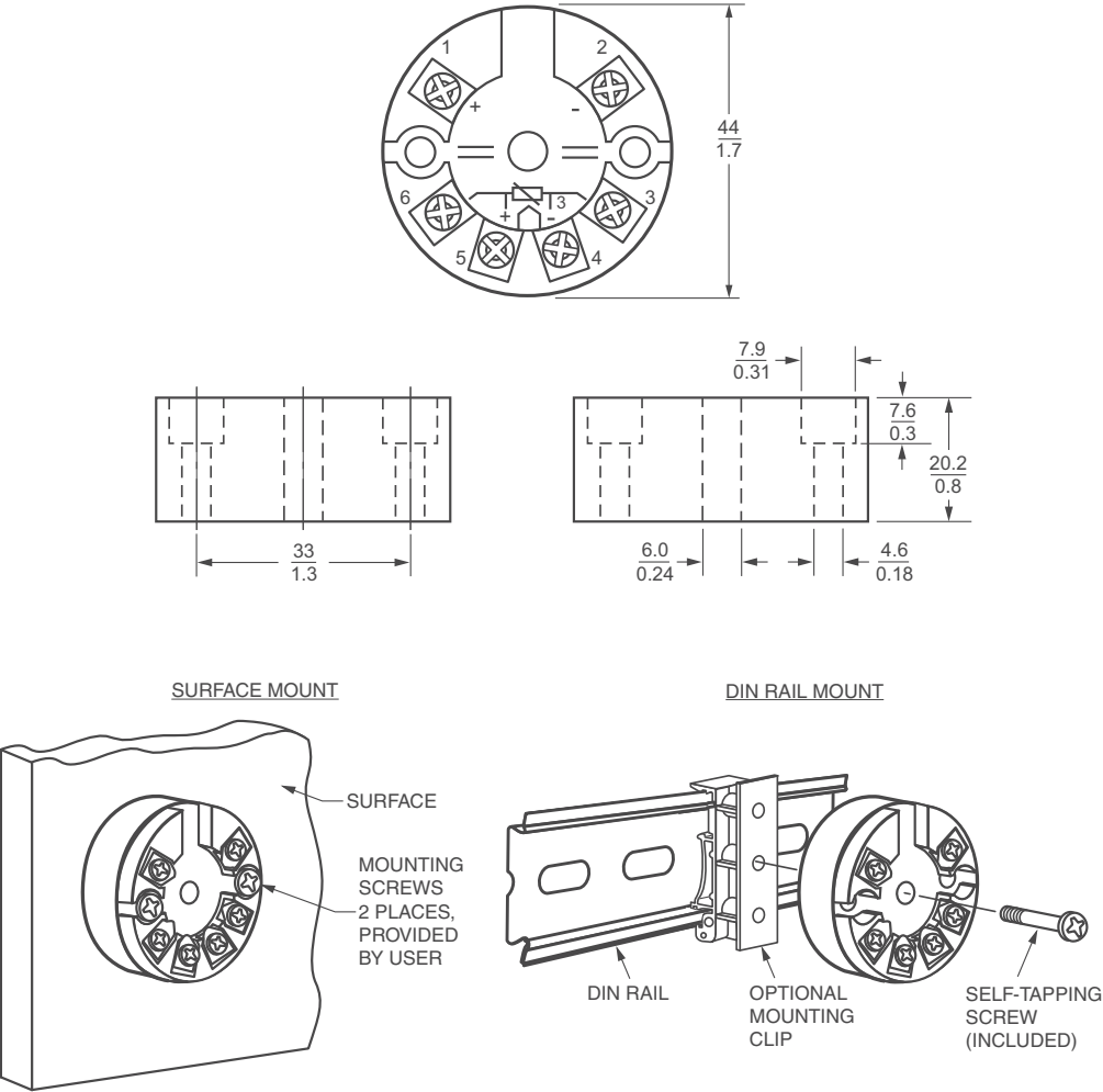
Figure 11 - Basic Transmitter — No Housing
